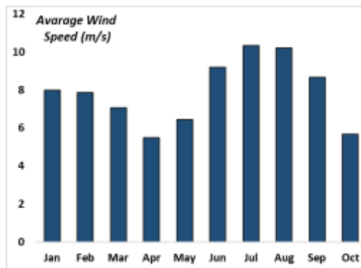
Figure 3. Monthly variation of the mean wind speed
