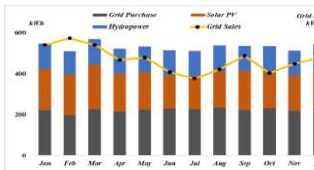
Figure 9. Monthly average electric production for the period of one year
