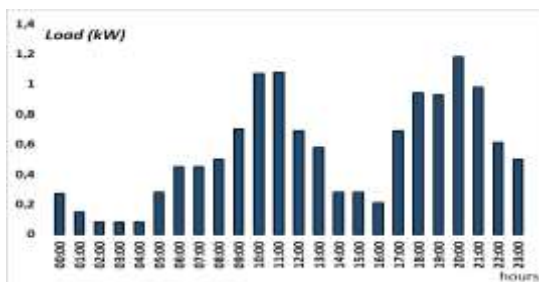
Figure 5. Typical daily electricity demand profile of the household in Somalia.
