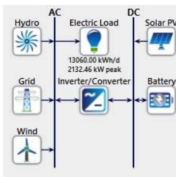
Figure 8. Schematic diagram of the on-grid hybrid system
