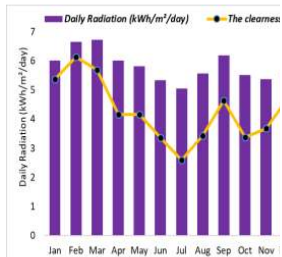
Figure 2. Averaged solar irradiance and clearness index for the selected area
