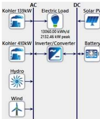
Figure 10. Schematic diagram of the off-grid hybrid system
