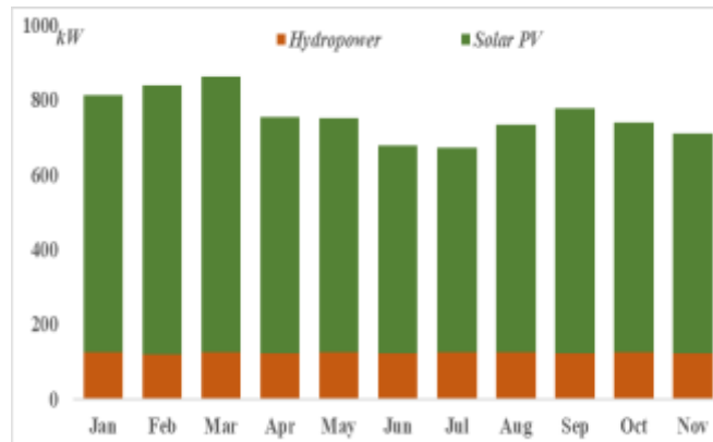
Figure 11. Monthly average electric production for the period of one year
