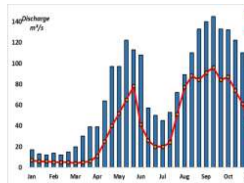
Figure 4. Long-term flow statistics of Shabelle River (m³/s)
