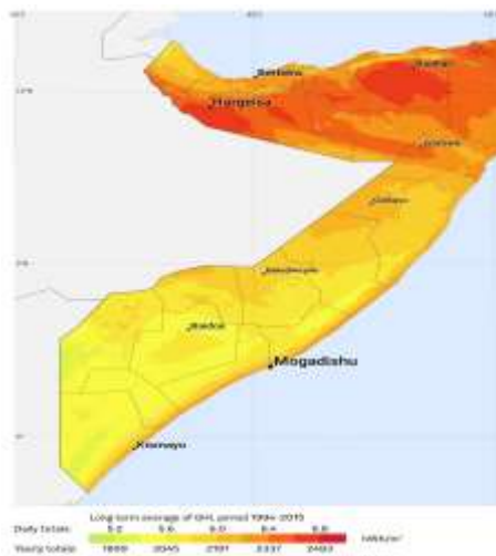
Figure 1. Solar radiation map of Somalia ( Solar Maps of Somalia , 2021)
