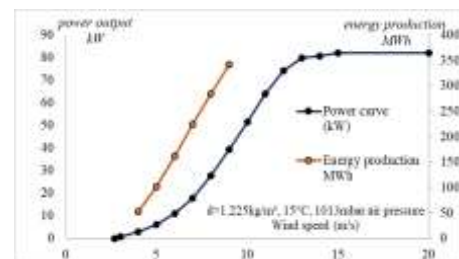
Figure 6. The energy production curve and the power-speed curve of the wind turbine
