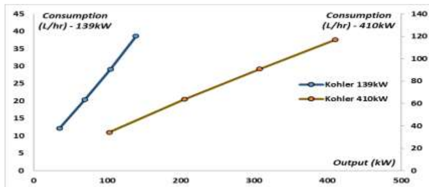
Figure 7. The fuel consumption curve of diesel generators
