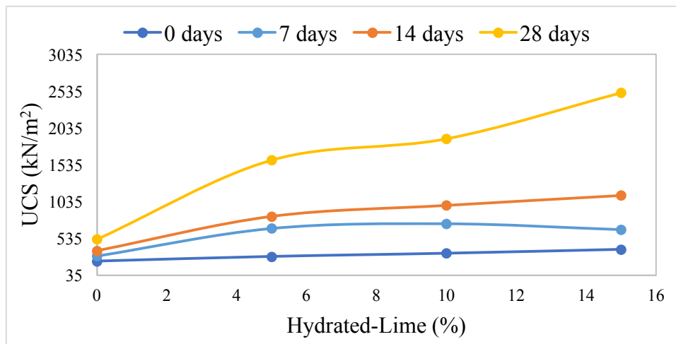
Figure 4. Hydrated-lime and curing period impacts (at 50° C) on unconfined compressive strength.
