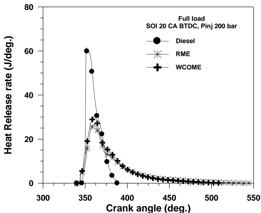
Figure 17 The heat release rate versus crank angles for different types of fuels
