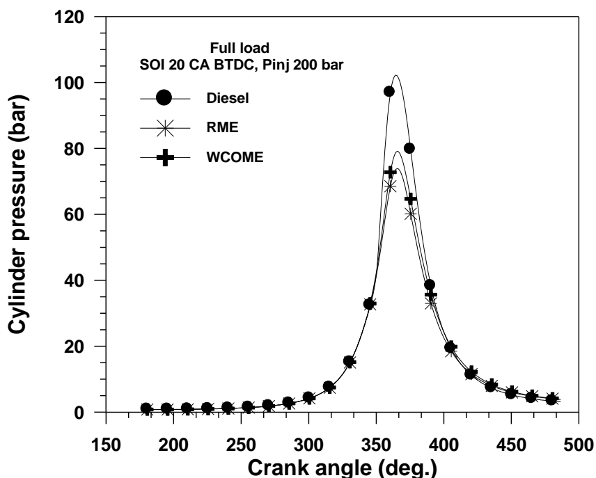
Figure 16 The cylinder pressure versus crank angles for different types of fuels
