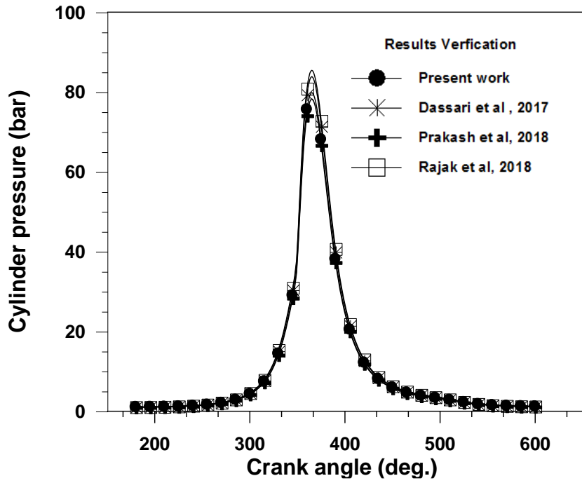
Figure 3 Verification of the cylinder pressure between different research papers.
