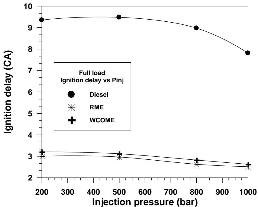
Figure 14 The ignition delay at different injection pressures for different types of fuels
