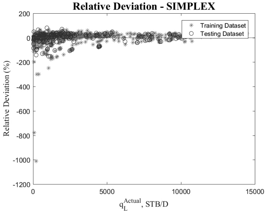
Figure 9. Relative Deviation plot for the SIMPLEX Developed Model (Training and Testing).
