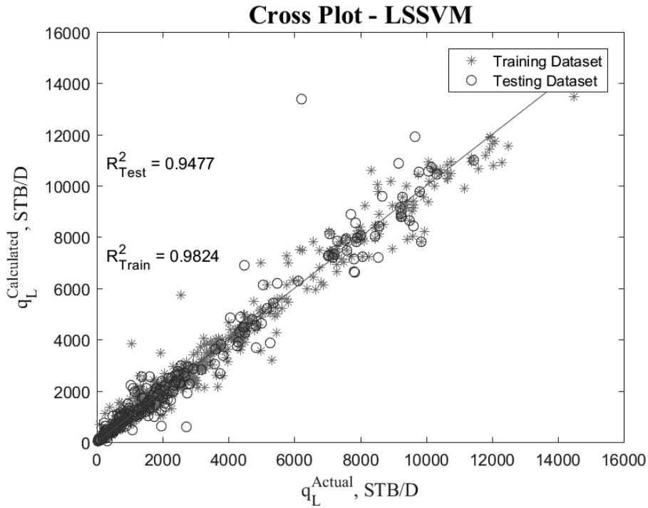
Figure 5. Cross plot for the LSSVM Developed Model (Training and Testing).
