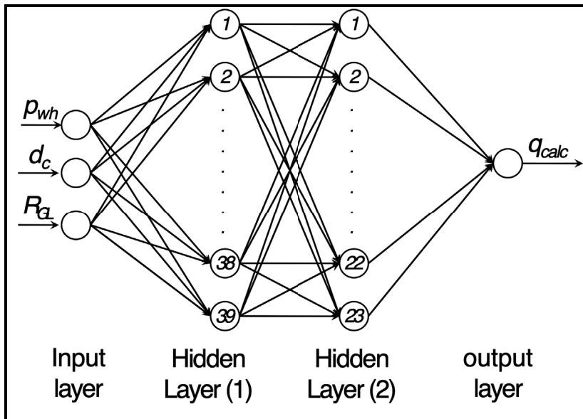
Figure 1. The structure of the ANN model.
