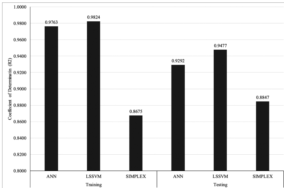
Figure 3. R^2 Comparison for Developed Models for both Training and Testing Datasets.
