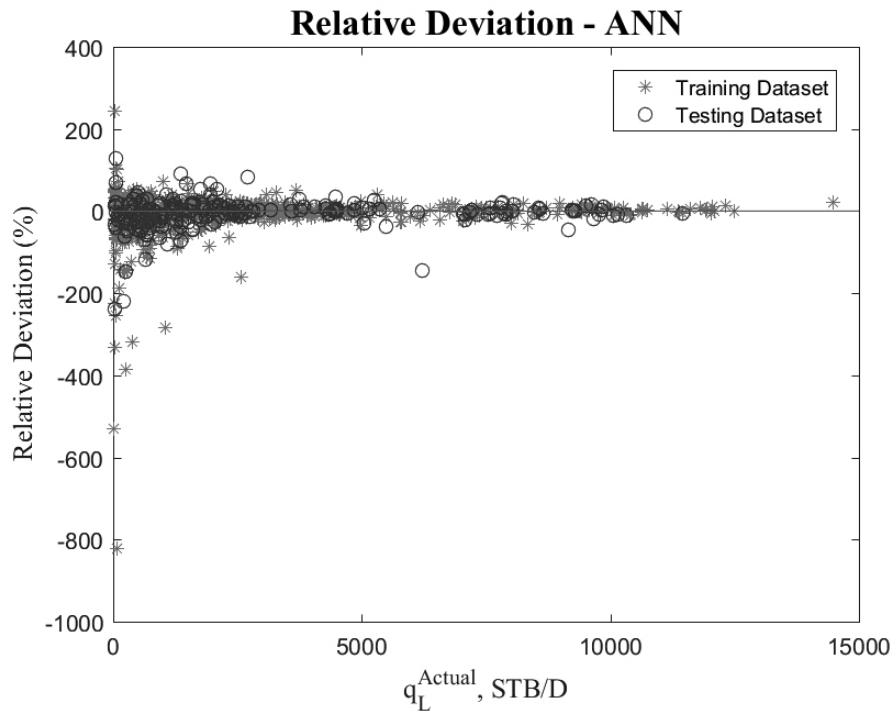
Figure 7. Relative Deviation plot for the ANN Developed Model (Training and Testing).
