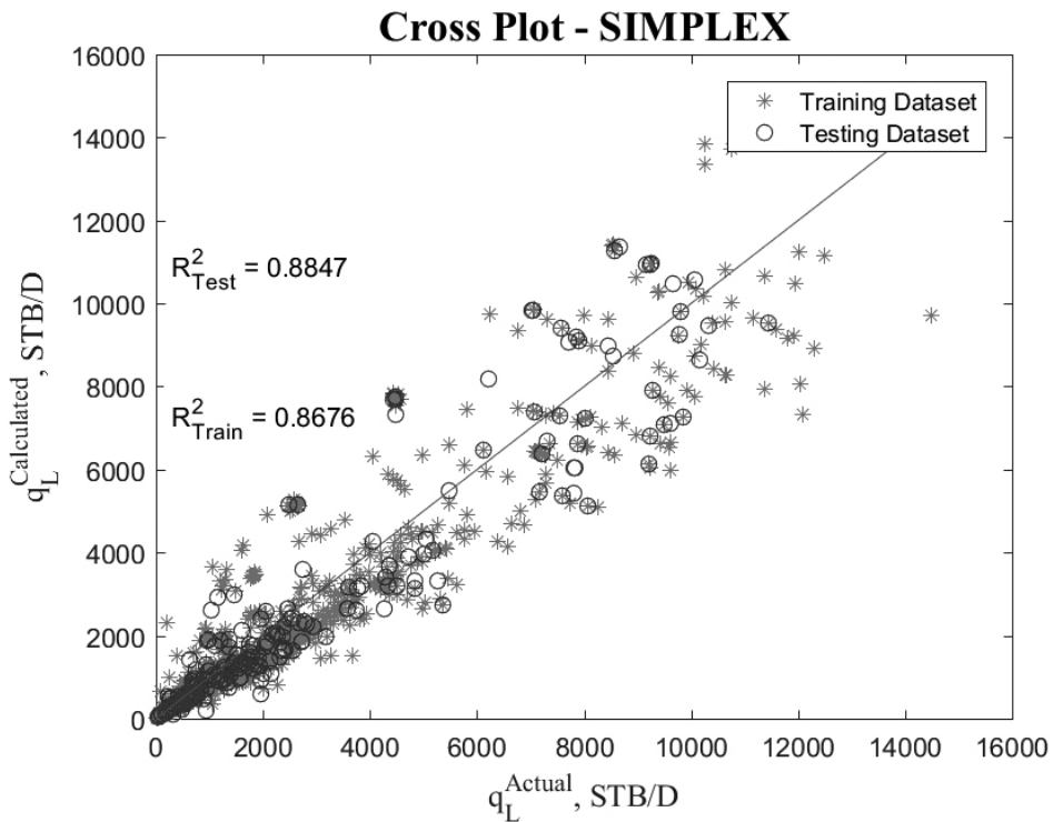
Figure 6. Cross plot for the SIMPLEX Developed Model (Training and Testing).
