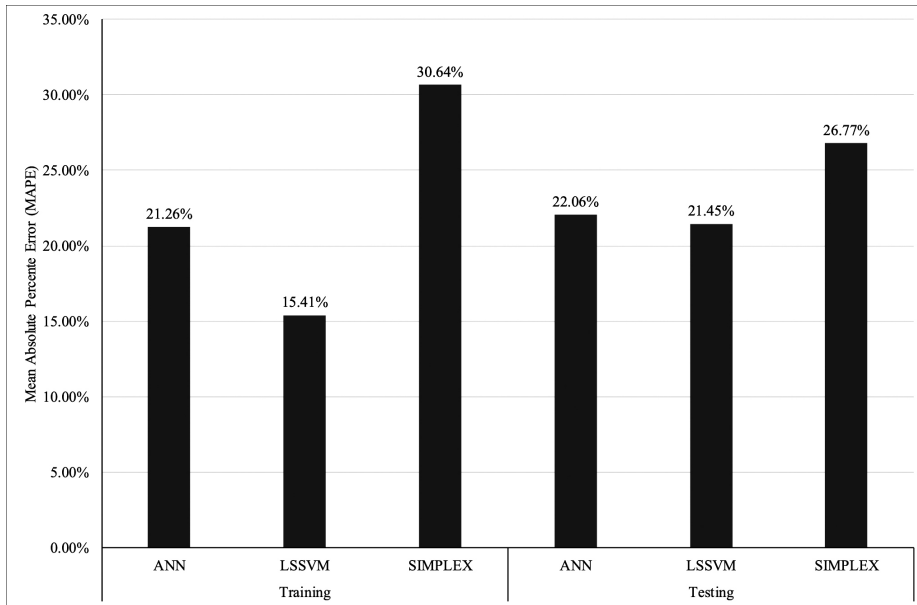
Figure 2. MAPE Comparison for Developed Models for both Training and Testing Datasets.
