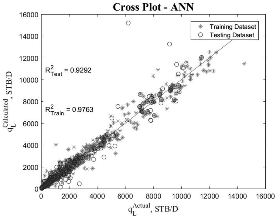
Figure 4. Cross plot for the ANN Developed Model (Training and Testing).
