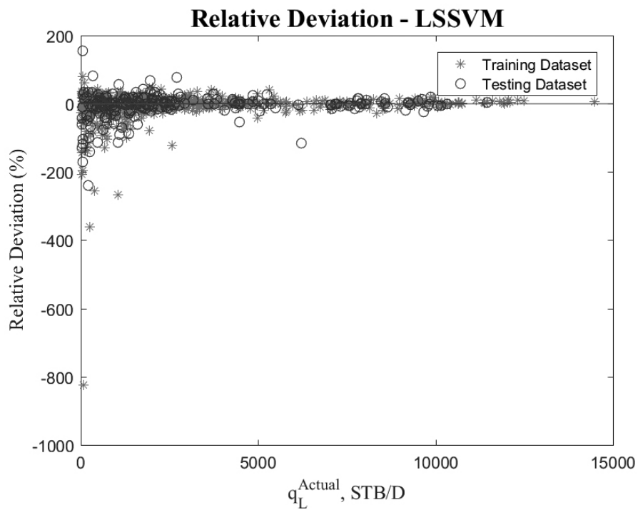
Figure 8. Relative Deviation plot for the LSSVM Developed Model (Training and Testing).
