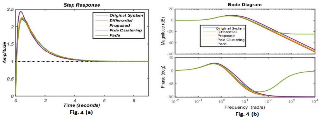
Figure 4 (a) Comparison of Step Responses with original & reduced System (Example:4), (b) Comparison of Bode Responses with original & reduced System (Example:4)
