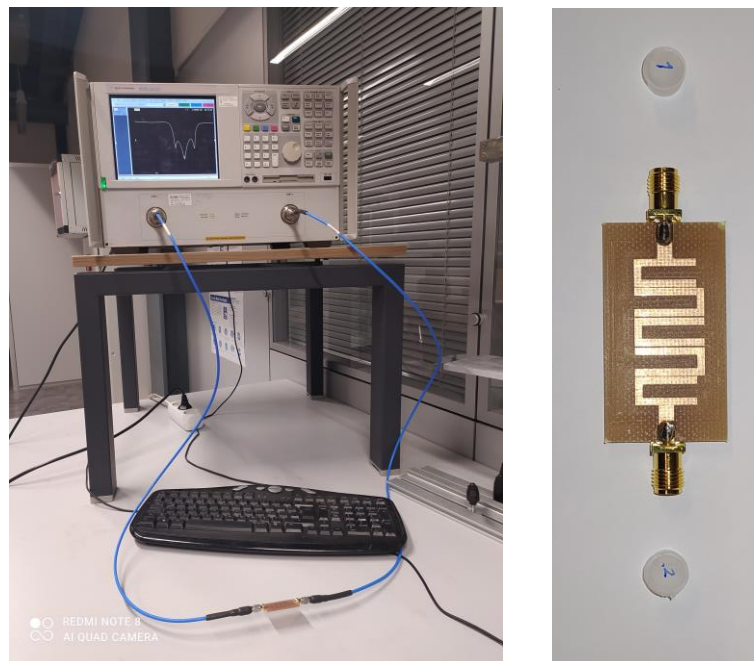
Figure 4 The manufactured and tested proposed microstrip hairpin bandpass filter
