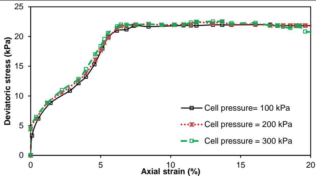
Figure 2. Stress-strain curves were obtained from unconsolidated undrained triaxial tests.
