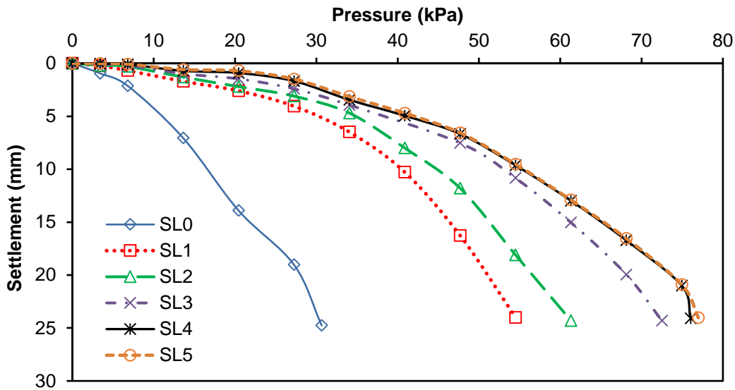
Figure 6. Settlement versus pressure for soil samples reinforced with several patterns of floating stone columns.
