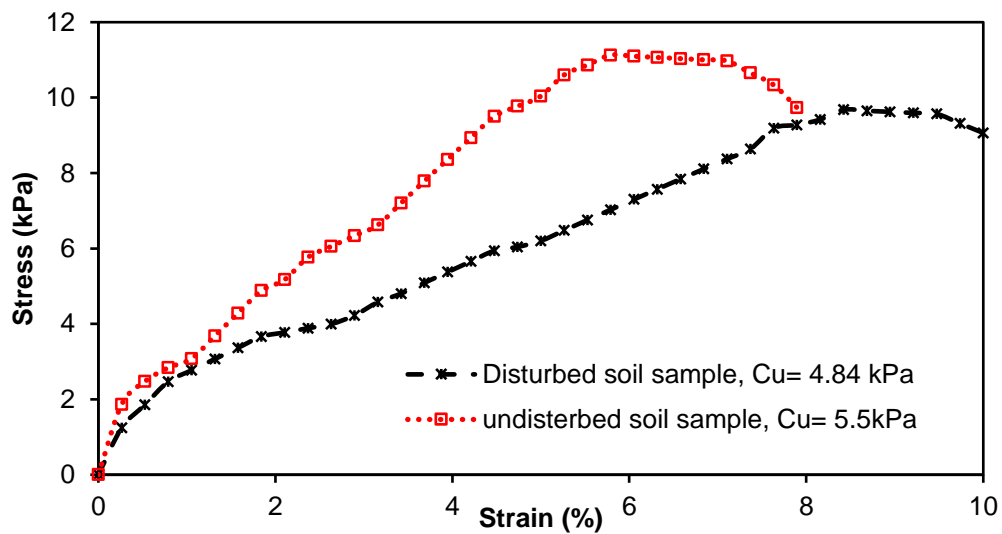
Figure 1. Stress-strain curves were obtained from unconfined compressive strength tests.
