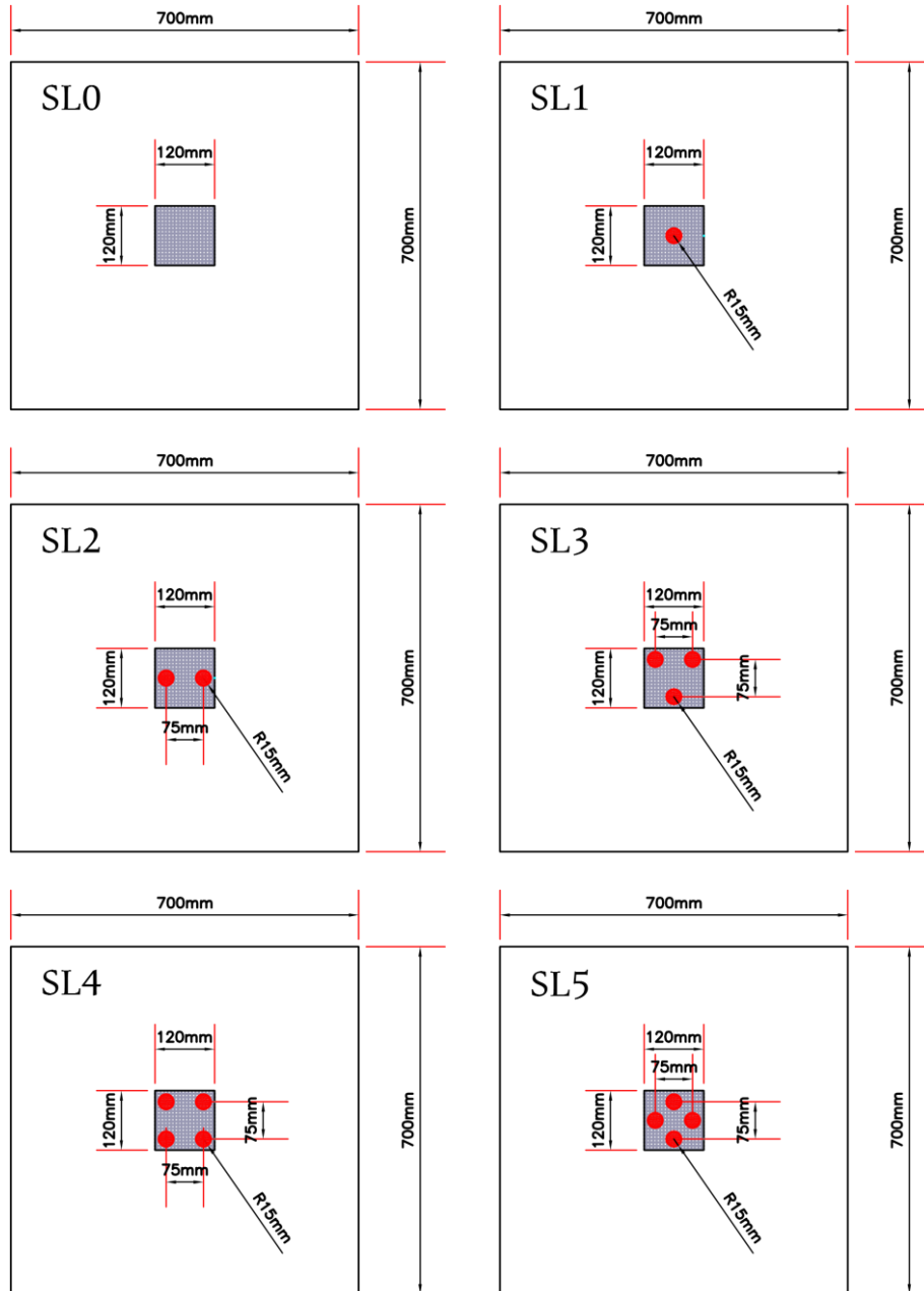
Figure 5. Distributions patterns of stone columns under raft footing in soft soil.
