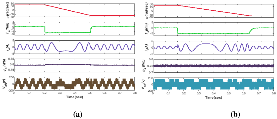
Figure 3. Speed reversal behavior at rated speed a) FCS-MPFOC b) MPTC
