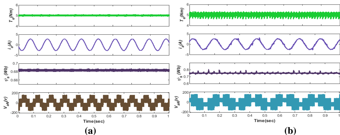
Figure 10. L_m mismatch analysis at load under rated speed a) FCS-MPFOC b) MPTC
