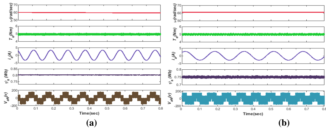
Figure 4. Full-load performance authentication at rated speed a) FCS-MPFOC b) MPTC
