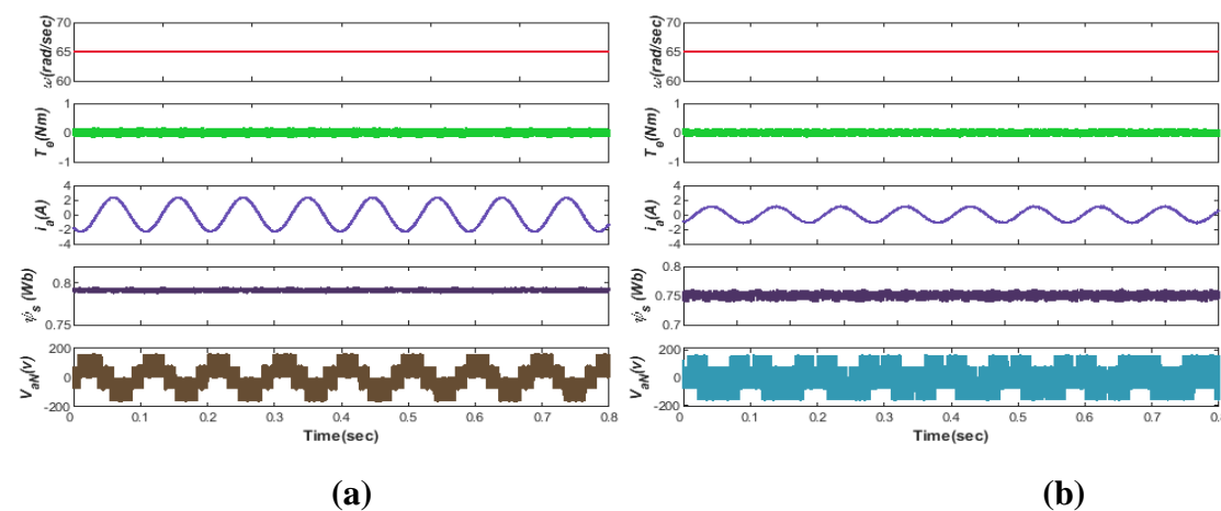
Figure 5. Steady-state analysis at rated speed a) FCS-MPFOC b) MPTC
