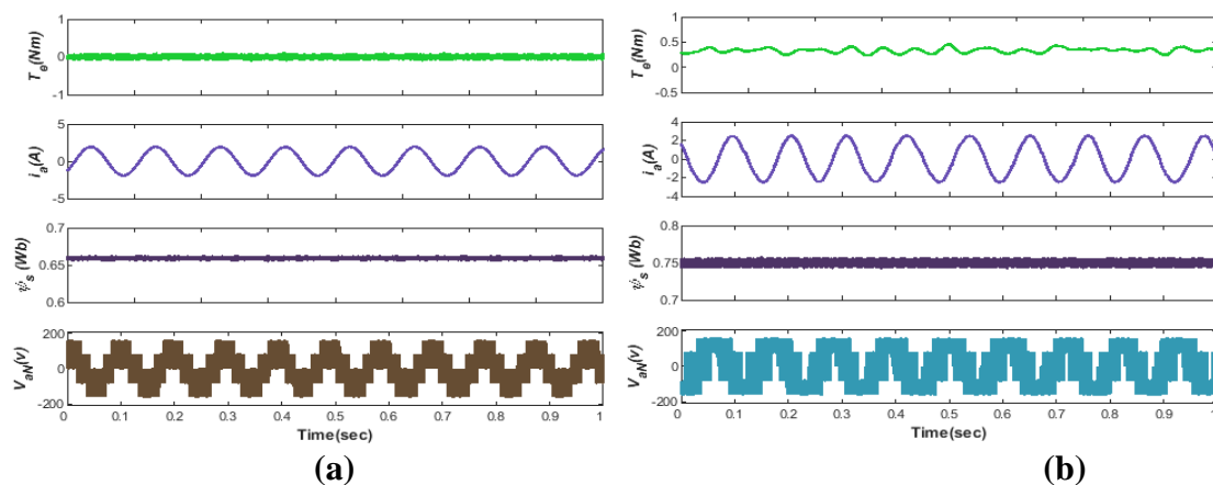
Figure 9. L_m mismatch analysis at no-load rated speed a) FCS-MPFOC b) MPTC
