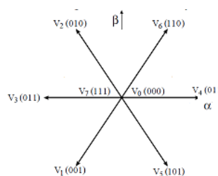
FIGURE 1b- 2L-VSI output voltage vector's
