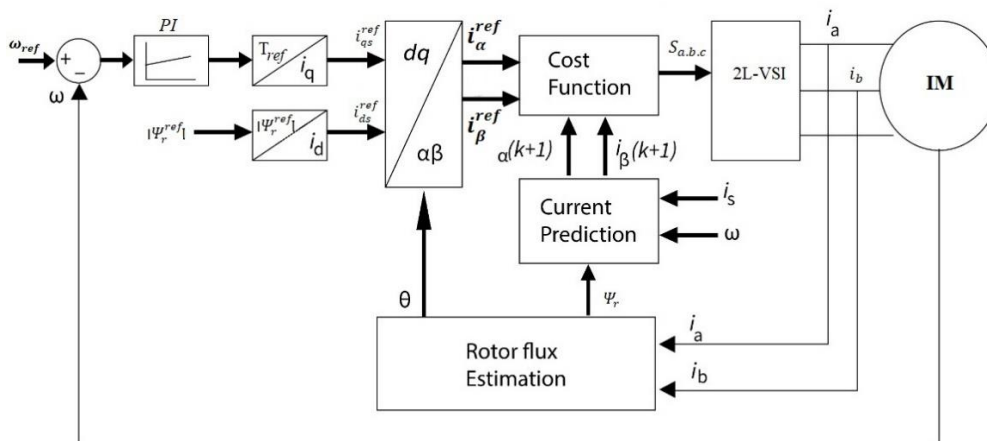
Figure 2. FCS-MPFOC for three-phase IM
