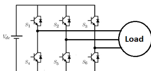
FIGURE 1a- 2L-VSI
