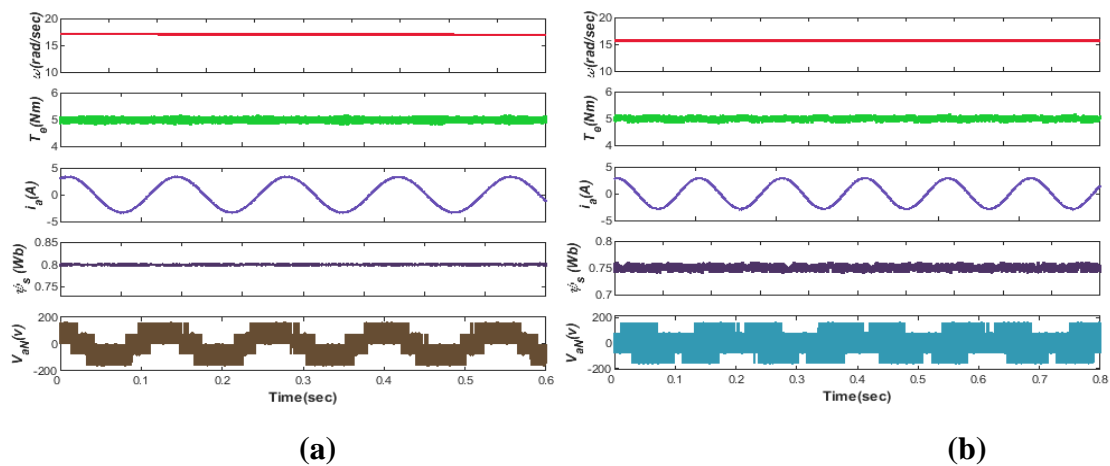
Figure 6. Performance validation at low speed a) FCS-MPFOC b) MPTC
