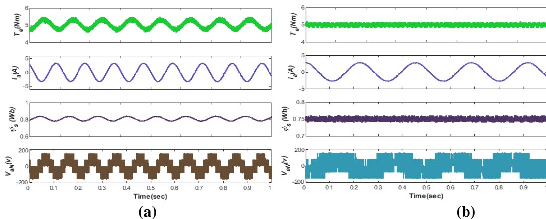
Figure 8. R_s variation validation at load under full speed a) FCS-MPFOC b) MPTC
