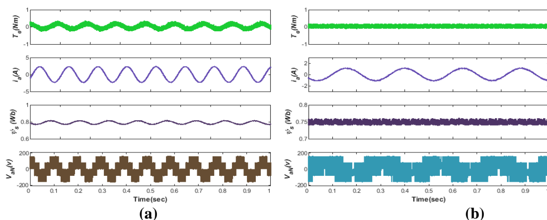
Figure 7. R_s sensitivity analysis at zero-load under rated speed a) FCS-MPFOC b) MPTC
