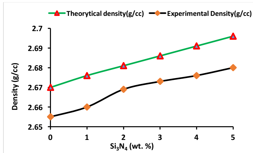
Figure 4 Density variation of Al/Si 3 N 4 composites with wt. % of Si 3 N 4
