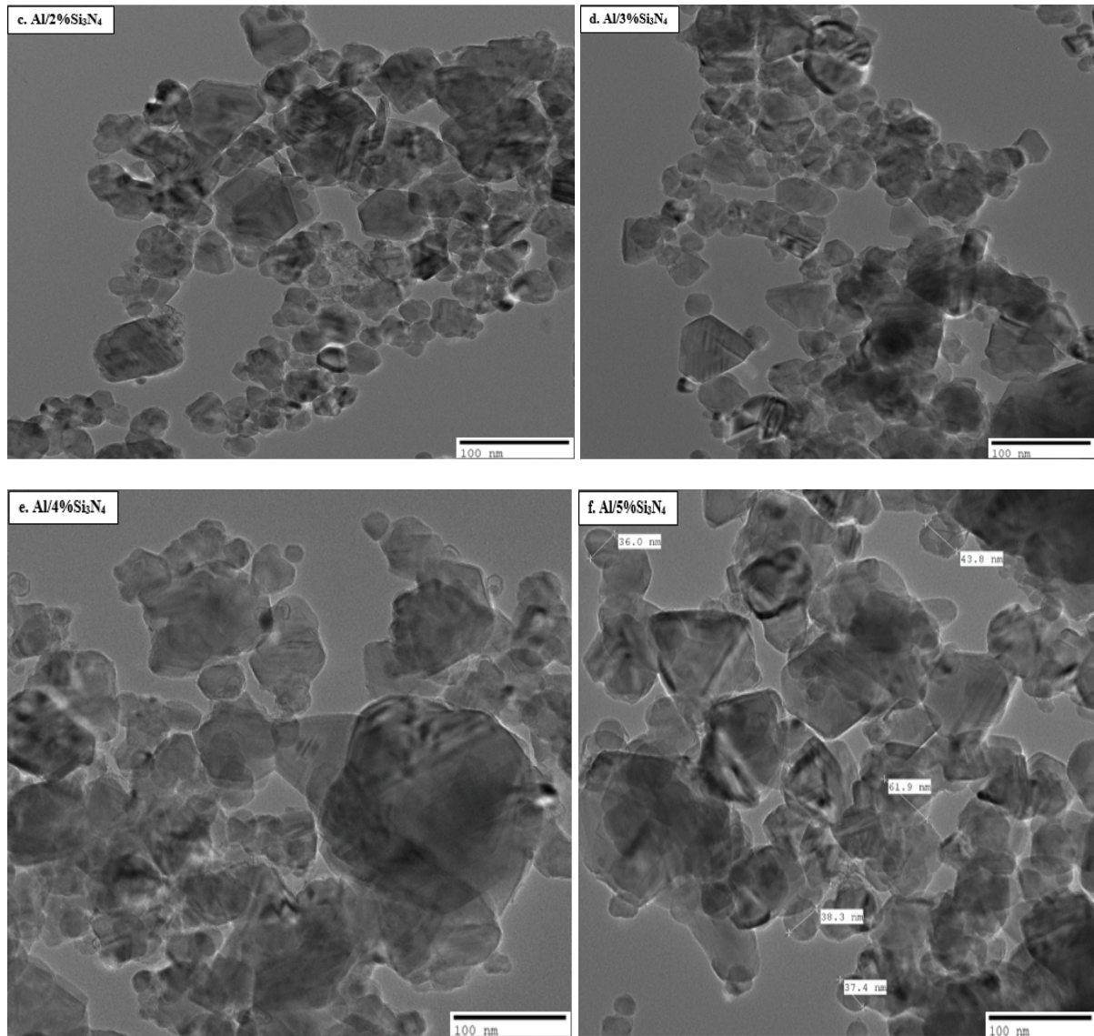
Figure 8(a-f) TEM images of Si 3 N 4 and stir cast Al/Si 3 N 4 nanocomposites
