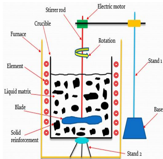
Figure 2 A block diagram of Stir Casting Set up
