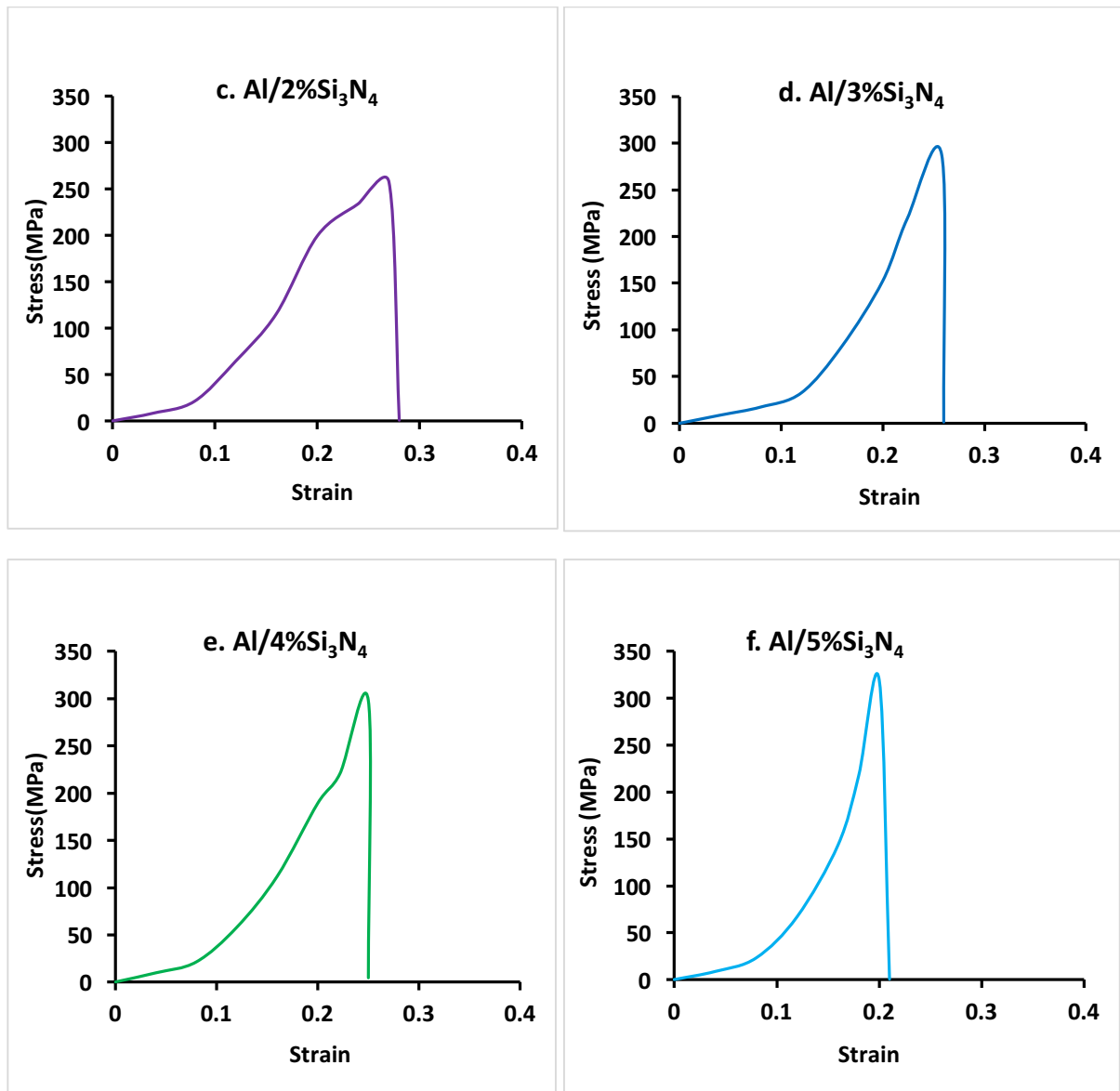
Figure 7(a-f) Tensile Stress Vs. Tensile Strain
