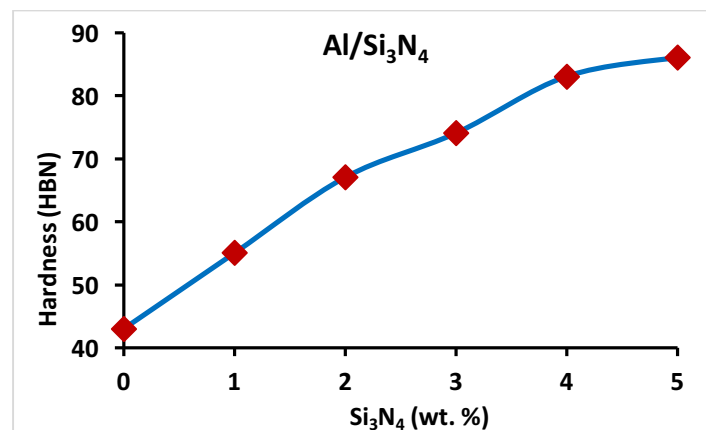
Figure 6 Hardness variation of Al/Si 3 N 4 composites with Si 3 N 4 particles
