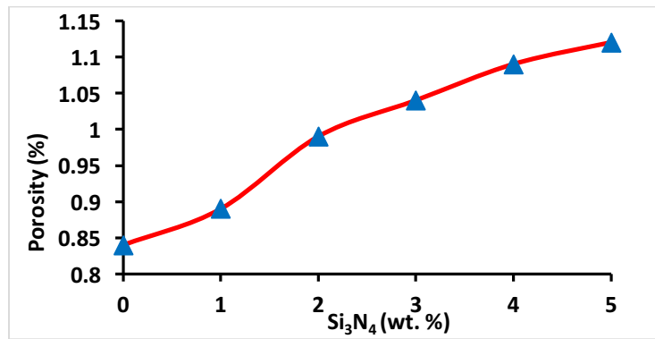
Figure 5 Porosity variation of Al/Si 3 N 4 composites with wt. % of Si 3 N 4
