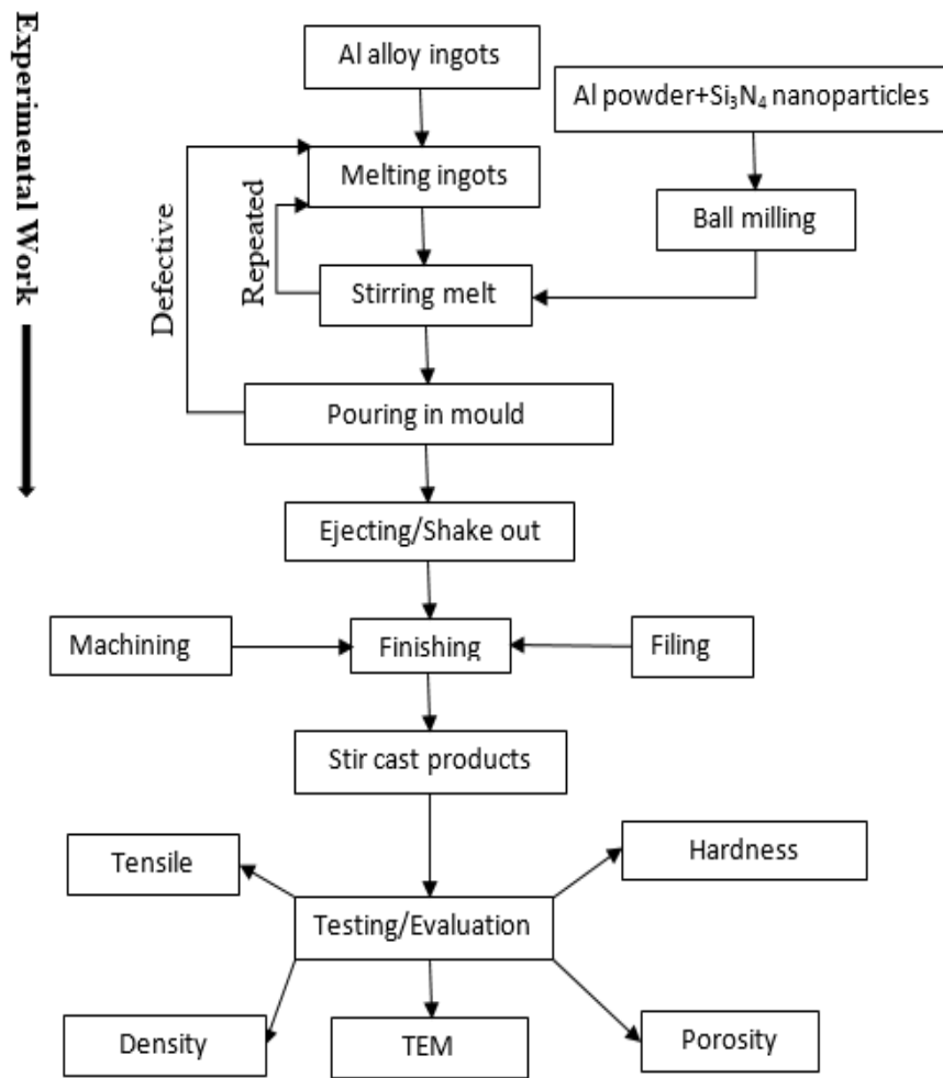
Figure 1 Steps for Preparation and testing of specimens
