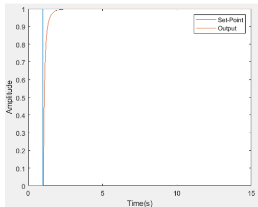
Figure 7 Unit Step Response of ACO tuned FOPID Controller ( M=150 )
