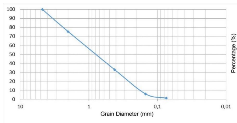
Figure 2. Grain size distribution curve of sandy soil.
