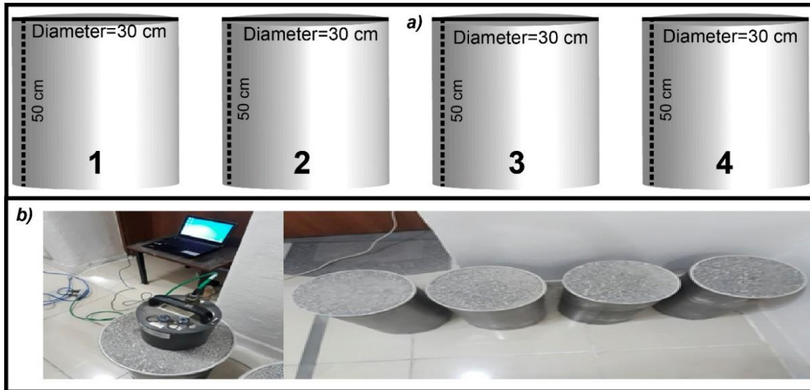
Figure 1 a. Cylinders created for current study. b. Experimental setup.
