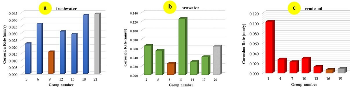
Figure 3. Corrosion rates of specimens in a) fresh water, b) sea water, and c) crude oil.
